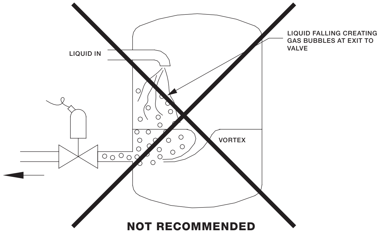
FIGURE 2: PIPING RECOMMENDATIONS
